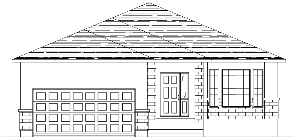
FRONT ELEVATION
